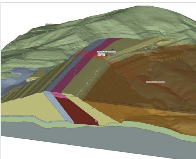
Safety and efficiency of a mine tailings facility is improved by using PLAXIS LE.
